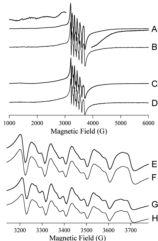
FIGURE 6: X-Band EPR spectra of Mn(II)-substituted forms of EcMetAP-I : (A) [Mn 2 (H79A EcMetAP-I )], (B) [MnMn(H79A EcMetAP-I )], (C) [Mn 2 (WT EcMetAP-I )], and (D) [MnMn(WT EcMetAP-I )]. The high- and low-field wings of the spectrum of [Mn 2 (H79A EcMetAP-I )] are shown with a larger (5 times) amplitude, above and below, respectively, trace A. Traces E–H are of the g_{\text{eff}} \sim 2 regions of spectra A–D, respectively. Spectra were recorded at 8 K with a microwave power of 0.2 mW, a field modulation amplitude of 1.2 mT, a modulation frequency of 100 kHz, and a sweep rate of 10.2 mT s -1 , and the samples were in 25 mM HEPES buffer and 150 mM KCl (pH 7).
