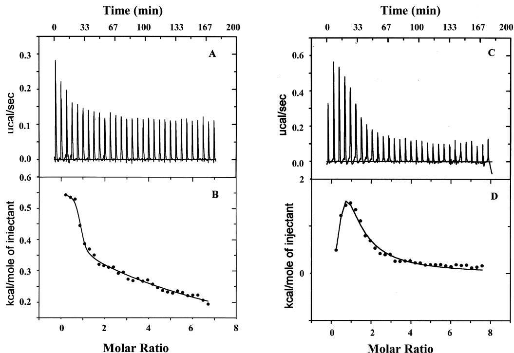
FIGURE 3: Isothermal titration calorimetry (ITC) titrations of 70 \mu M solutions of H79A EcMetAP-I with 5 mM Co(II) (A) or 5 mM Mn(II) (C). The best fits of the data in panels A and C are shown in panels B and D, respectively, after subtraction of the heat of dilution.
