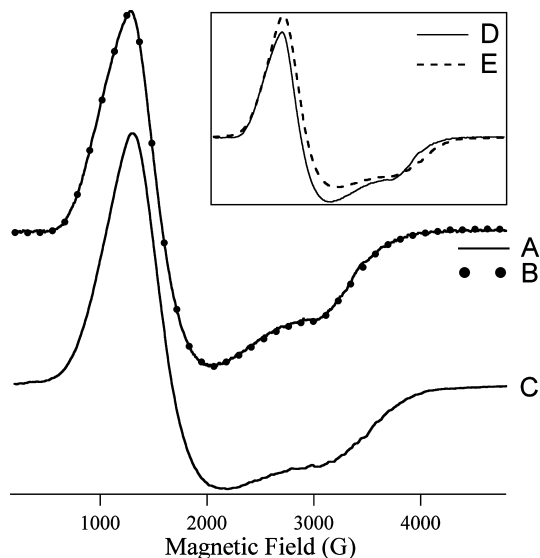
FIGURE 5: X-Band EPR spectra of Co(II)-substituted forms of EcMetAP-I : (A) [Co 2 (H79A EcMetAP-I )], (B) [CoCo(H79A EcMetAP-I )], and (C) [CoCo(WT EcMetAP-I )]. Spectra A and B were recorded at 8 K with a 0.2 mW microwave power; spectrum C was recorded at 9 K with a 0.2 mW microwave power. The amplitude of trace A is shown multiplied by 1.88 compared to spectrum B. The inset shows the spectra of [CoCo(H79A EcMetAP-I )] (D) and [CoCo(WT EcMetAP-I )] (E) overlaid. All the spectra were recorded at a field modulation amplitude of 1.2 mT, a modulation frequency of 100 kHz, and a sweep rate of 10.2 mT s -1 , and the samples were in 25 mM HEPES buffer and 150 mM KCl (pH 7.5).
